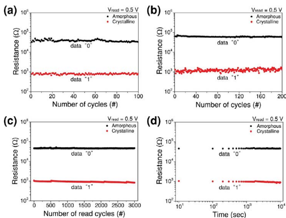
Figure 4. Device reliability evaluations. Write endurance of the PCM device (a) without and (b) with SiO x nanostructures (FF = 50%). (c) Read endurance and (d) retention time results of the PCM cells with SiO x nanostructures (FF = 50%).
